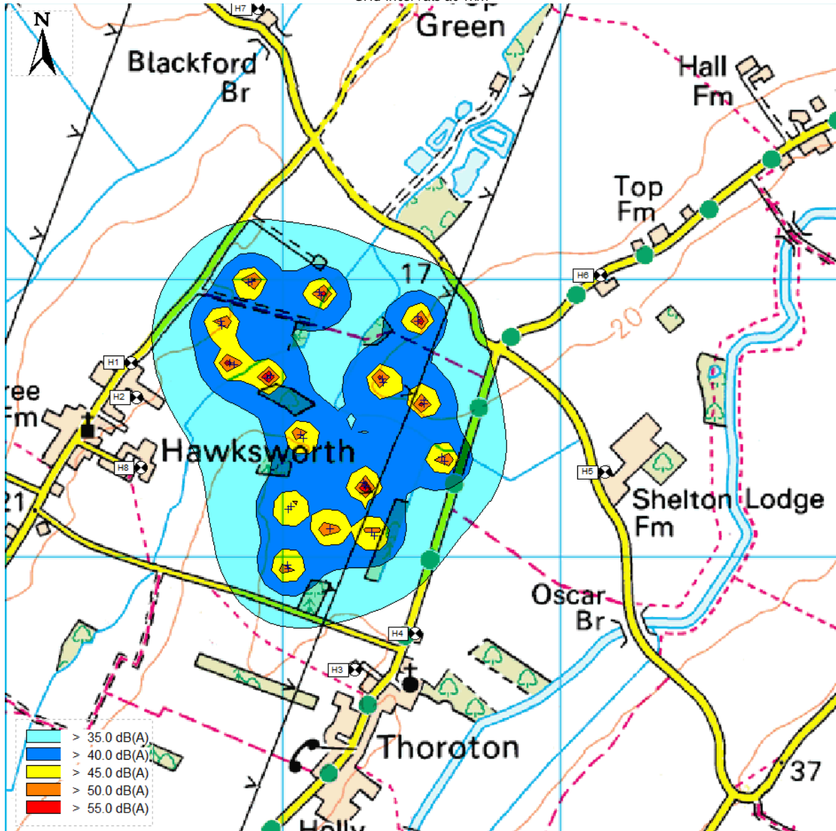
Figure 1 - Predicted Sound Footprint The L_{Aeq} descriptor has been used Grid intervals at 1km
